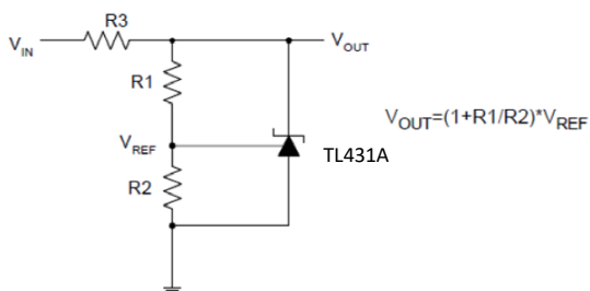
Shunt Regulator
