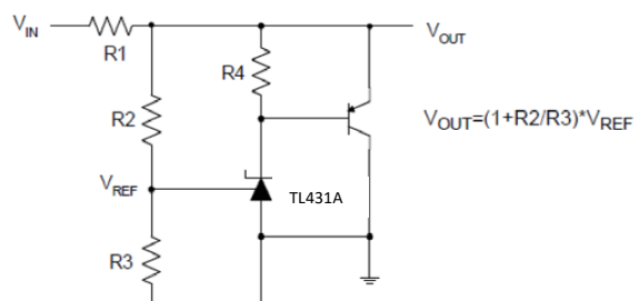
High Current Shunt Regulator
