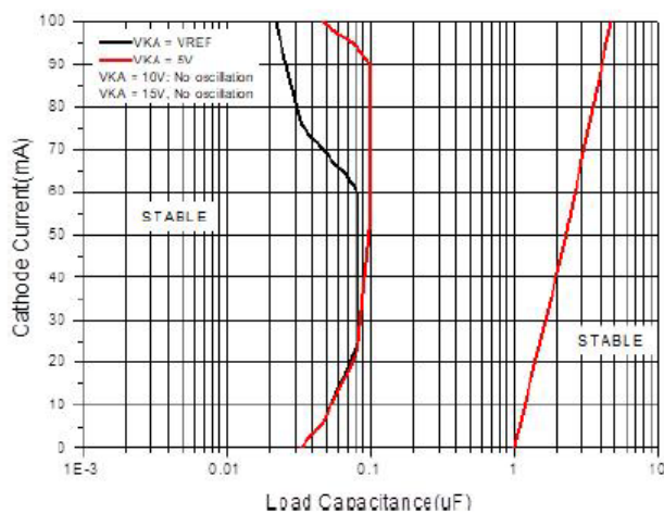
Stability Boundary Conditions vs. Load Capacitance
