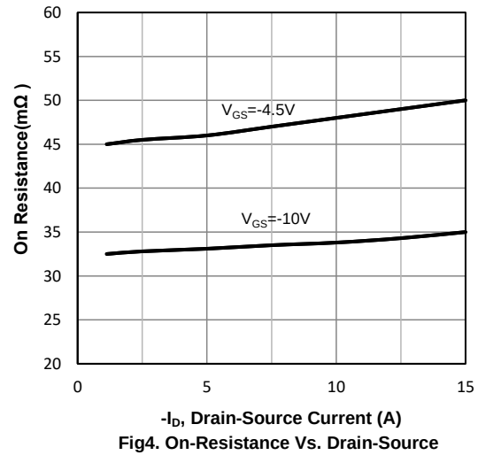
Fig4. On-Resistance Vs. Drain-Source
