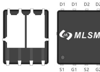
PDFN5X6-8L view
