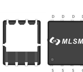
PDFN5X6-8L view
