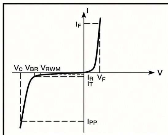
V-I characteristics for a uni-directional TVS
